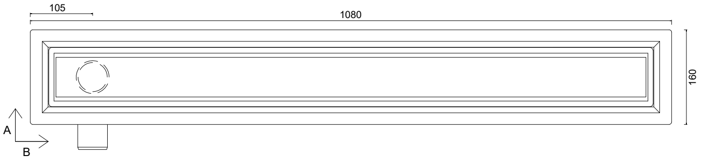
Plan View
