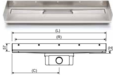
RIGHT & REAR WALL FLANGES / CENTRE OUTLET
