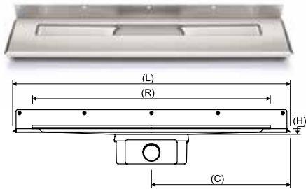
LEFT & REAR WALL FLANGES / CENTRE OUTLET
