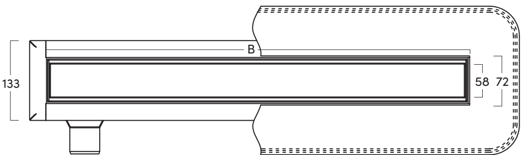
Plan View
