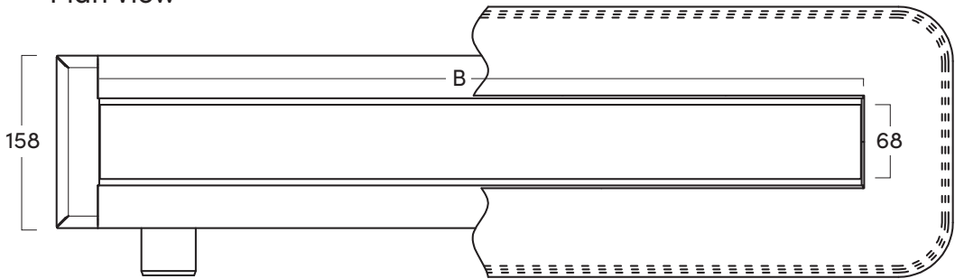
Plan View
