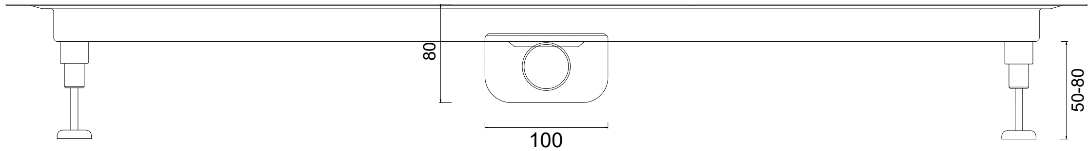
Section B
