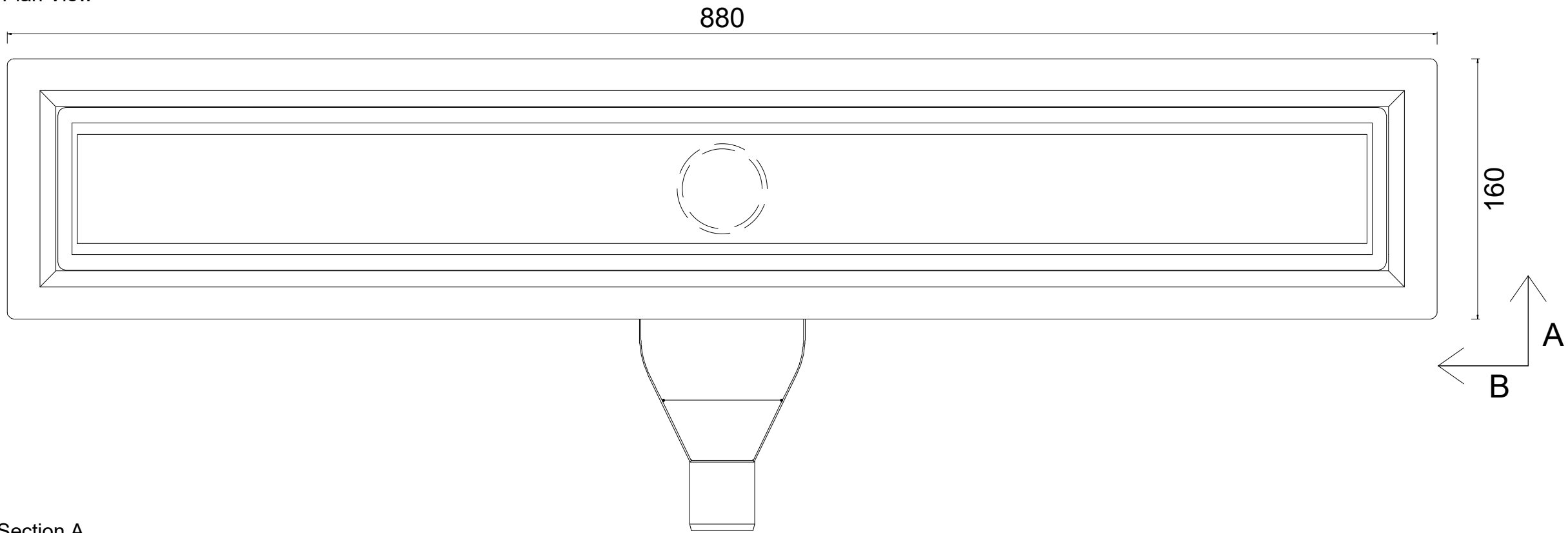
Section A
