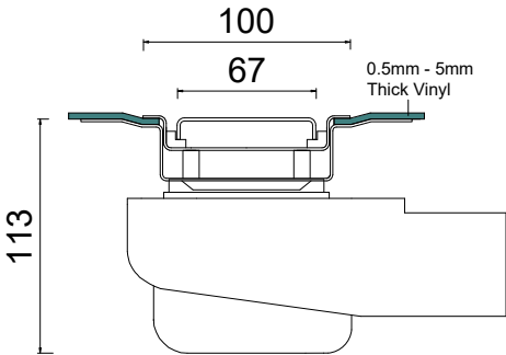
Section B
