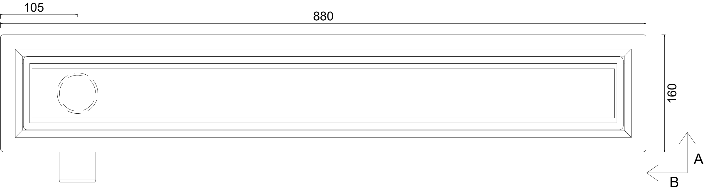
Plan View
