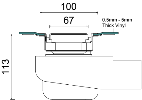
Section B
