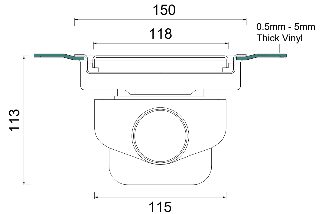
Side View
